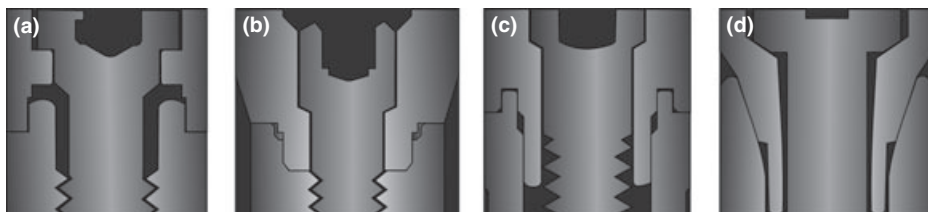
Fig. 1. Drawing showing the analyzed connections. (a) control group; (b) test group 1; (c) test group 2; (d) test group 3.
